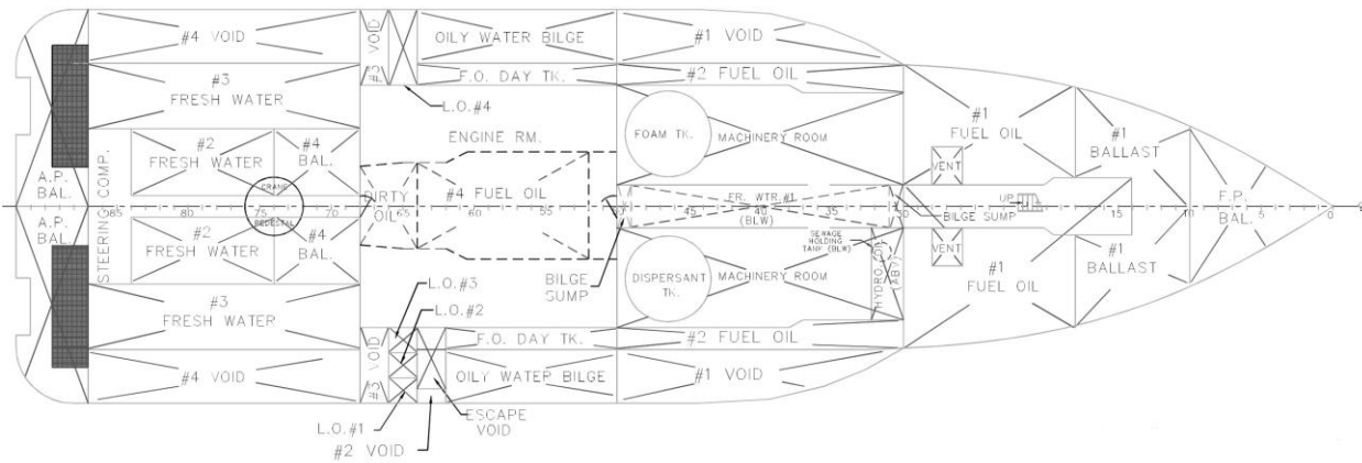
HOLD PLAN
